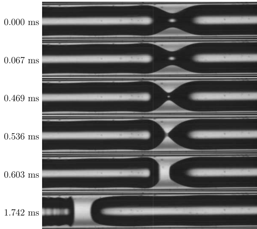
Figure 4.7. Lobe evolution and coalescence in a round channel, \theta \leq 20^\circ . The flow is from right-to-left and the width of the images is 3.455 mm.
