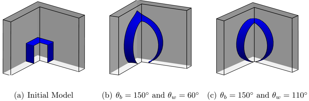
Figure 2.1. Initial and converged solutions for liquid that is in contact with the porous electrode (horizontal plane, contact angle \theta_b ) and two bipolar plate walls (contact angle \theta_w ) in a channel bend. The drops shown in 2.1(b) and 2.1(c) are the same volume.
