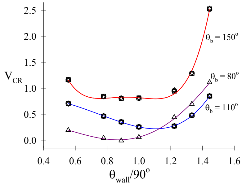
Figure 2.6. Critical plug volume in 1 \times 1 square channels for a range of bipolar plate channel contact angles \theta_w , three values of \theta_b corresponding to three different GDLs. The correlations shown (solid lines) correspond to equation 2.1 and Table 2.1 for the straight ( 2\alpha = 180^\circ ) channel. The family of curves shown in Figures 2.4 and 2.5 are obtained by adding 1/\tan(\alpha) .
