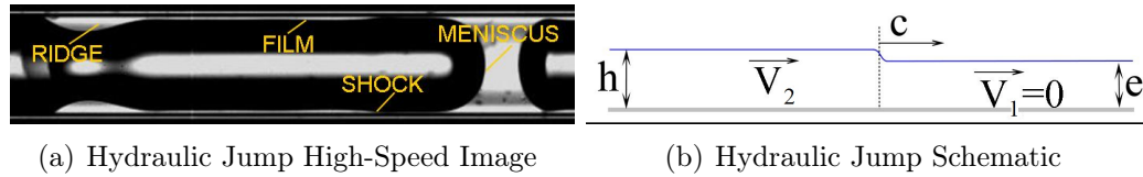
Figure 6.8. Hydraulic Jump in a Non-Wetting Film
