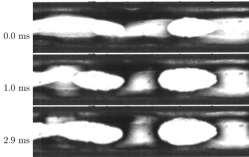
Figure 4.12. Film rupture in a square channel, \theta = 80^\circ . The flow is from right-to-left and the width of the images is 2.866 mm.
