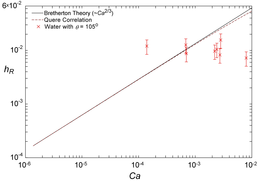
Figure 5.4. Non-dimensional film thickness vs. Ca , the nonwetting case.
