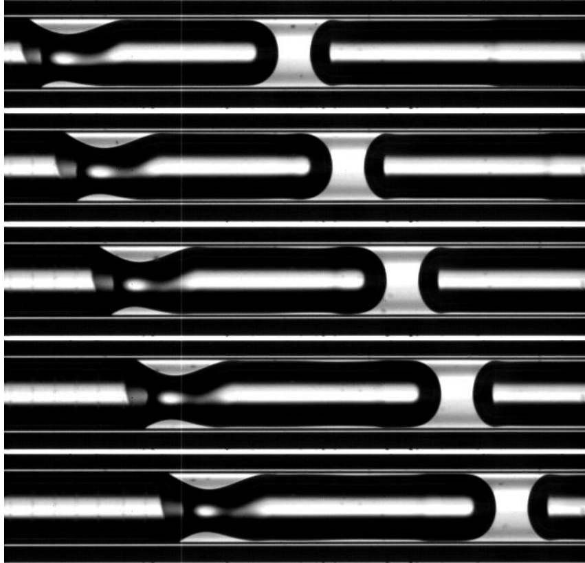
Figure 6.7. Non-wetting Supercritical Taylor bubble (with hydraulic jump), Ca = 0.00357 . (U - U_{CL})/c^* = 0.95 . Images 2 ms apart. The width of the images is 5.74 mm.
