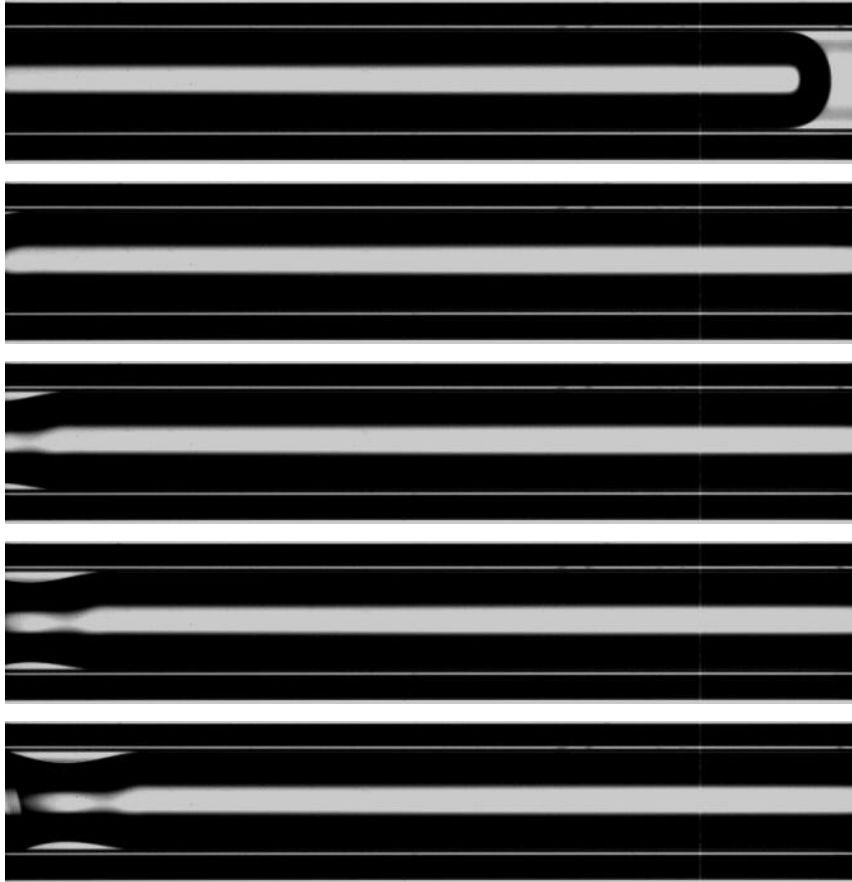
Figure 6.4. Wetting Taylor bubble , Ca = 0.0034 . Images 4 ms apart. The width of the images is 5.74 mm.
