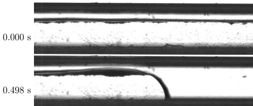
Figure 4.11. Slug flow in a square channel, \theta = 80^\circ . The flow is from right-to-left and the width of the images is 2.866 mm.
