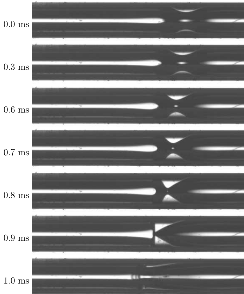
Figure 4.4. Lobe formation and collapse in a square channel, \theta \leq 20^\circ . The flow is from right-to-left and the width of the images is 3.931 mm.
