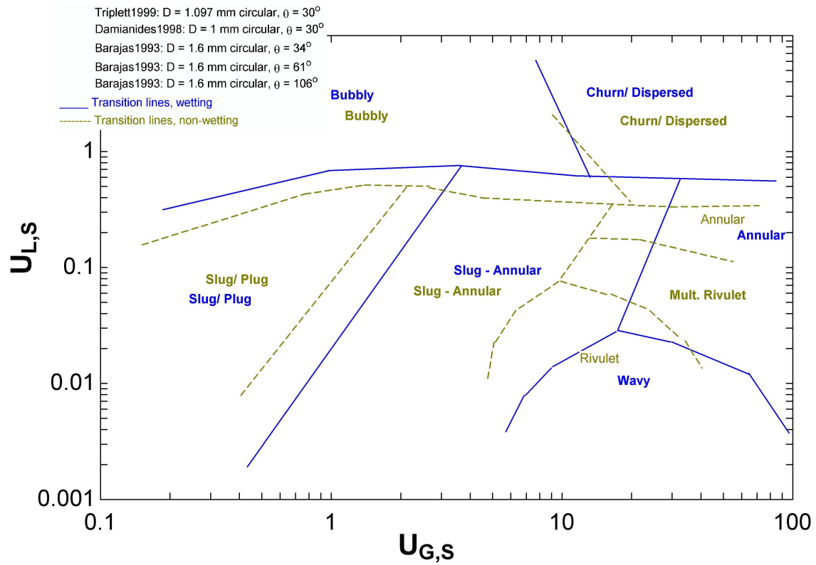
Figure 4.1. Two-Phase Transitions in Round Microchannels [1–3]
