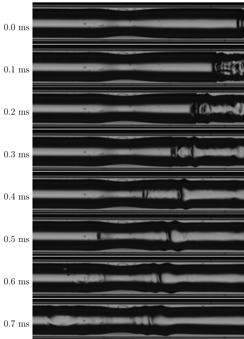
Figure 4.9. Lens formation and collapse in a round channel, \theta = 105^\circ . The flow is from right-to-left and the width of the images is 6.513 mm.
