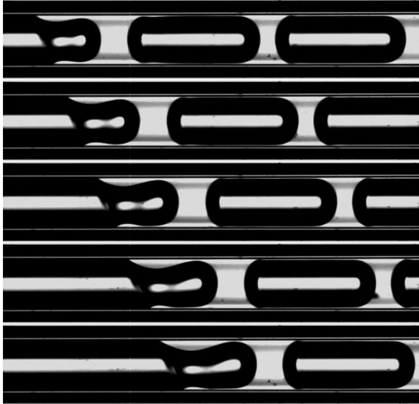
Figure 6.5. Non-wetting Taylor bubble , Ca = 0.0037 . The images are captured every 2 ms. The width of the images is 5.74 mm.
