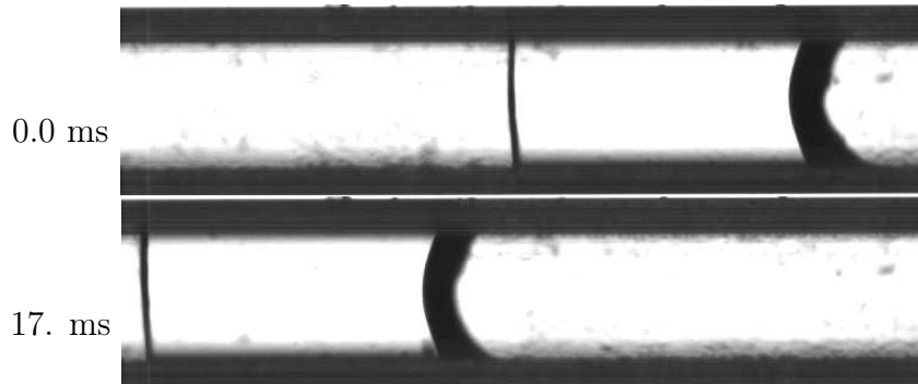
Figure 4.10. Plug flow in a square channel, \theta = 80^\circ . The flow is from right-to-left and the width of the images is 2.866 mm.
