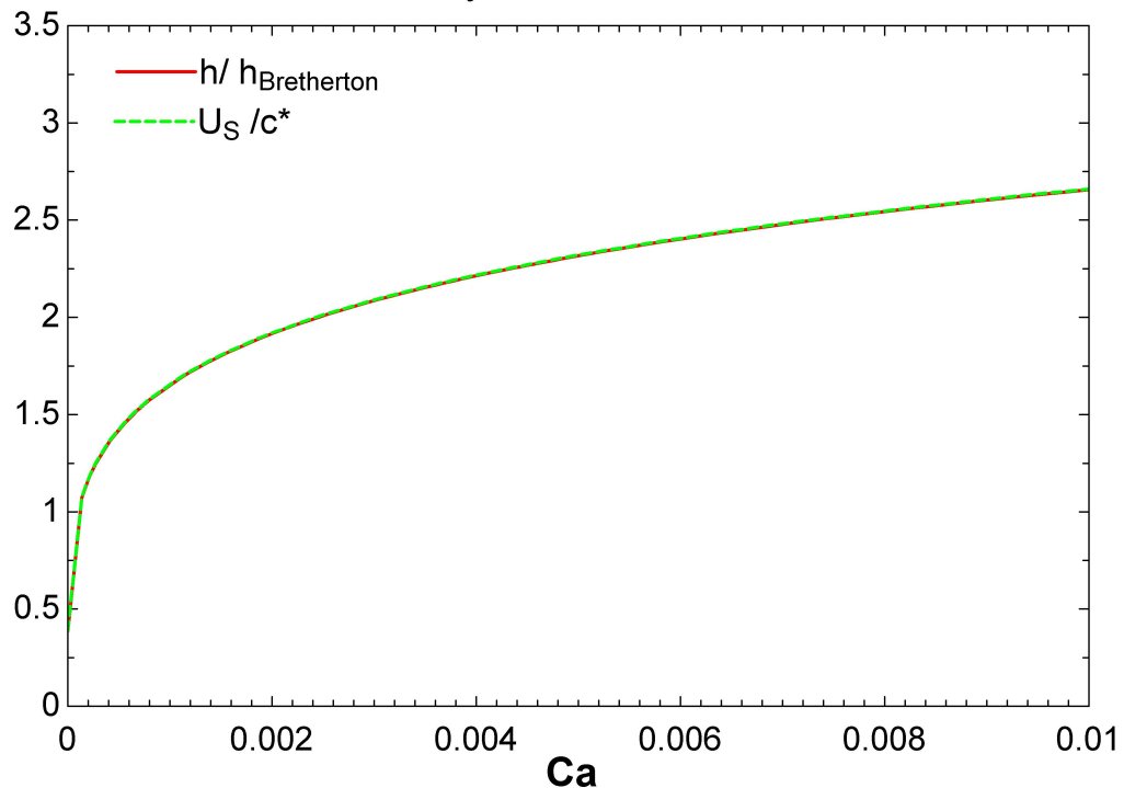
Figure 6.14. The Actual to Bretherton Film Thickness Ratio, and the Shock to Critical Velocity Ratio as a Function of Capillary Number. Note that the two lines coincide.
