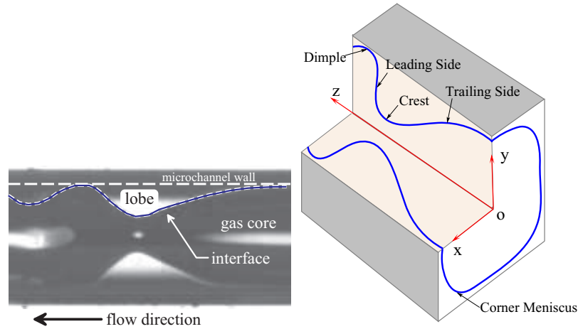
(a) Image of lobe formation detail- (b) Schematic of lobe formation in the leading and trailing sides of the microchannel the interface.
