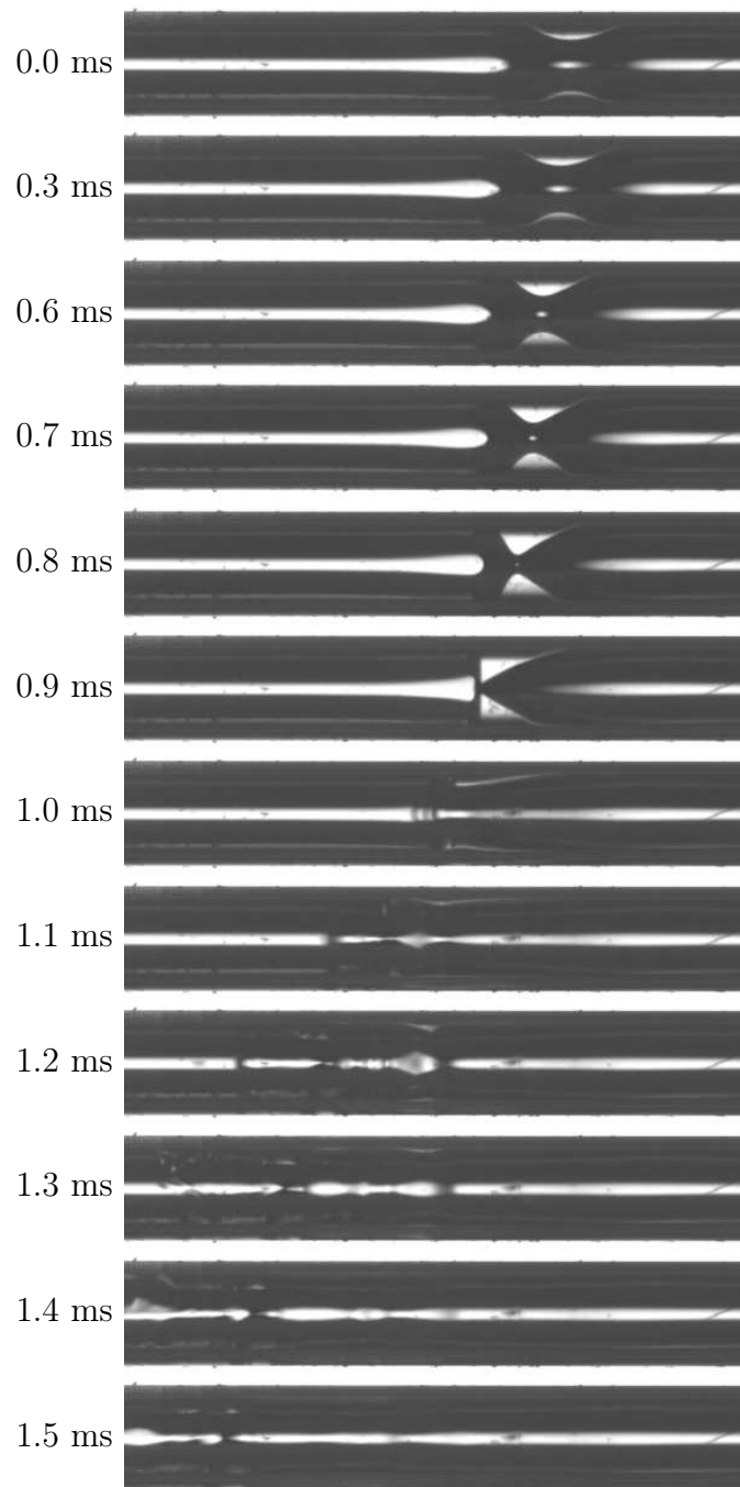
Figure 3.2. Sequence of lobe formation and collapse. The flow is from right-to-left and the width of the images is 3.931 mm.
