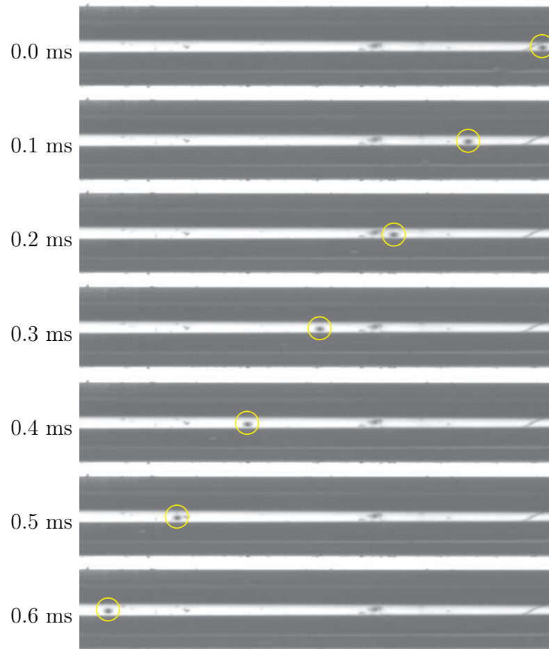
Figure 3.7. Sequence the motion of a liquid drop in the gas phase. The liquid drop is marked with a circle. The velocity of the drop is 6 m/s. The width of the images is 3.931 mm.
