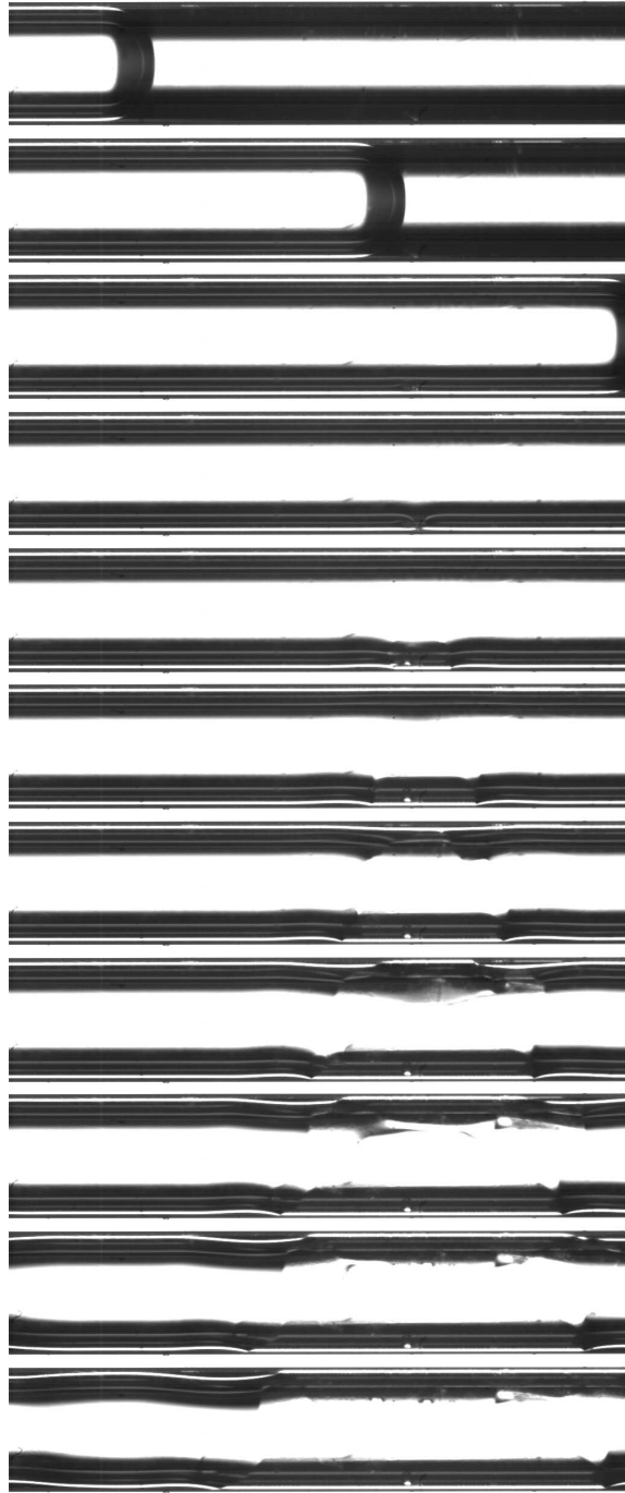
Figure 5.5. Viscous film deposition in a nonwetting capillary, \theta = 105^\circ . Image width of 4.427 mm. Consecutive images 8.032 ms apart.
