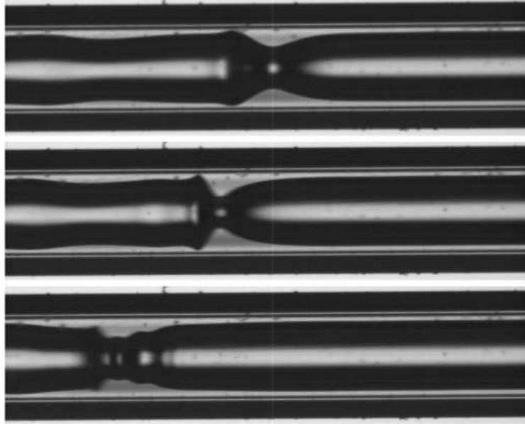
Figure 4.6. Lobe formation and collapse in a round channel, \theta \leq 20^\circ . Consecutive frames 0.067 ms apart. The flow is from right-to-left and the width of the images is 3.438 mm.
