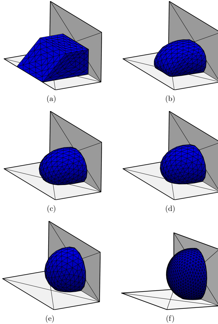
Figure 2.9. Energy minimization steps towards an equilibrium configuration (f). The base (GDL) contact angle is \theta_b = 150^\circ and the channel wall contact angle is \theta_w = 100^\circ .
