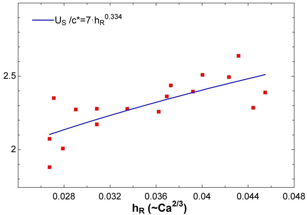
Figure 6.11. Non-dimensional Shock Velocity Correlation
