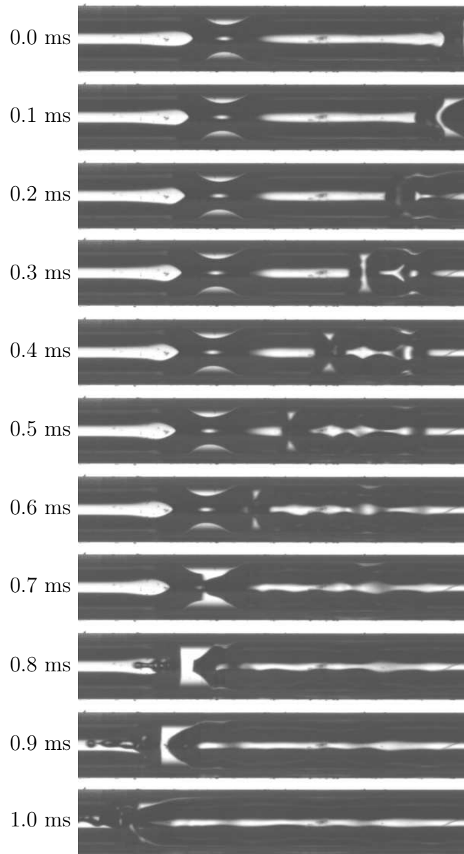
Figure 3.5. A 1-ms sequence of images showing lobe-lobe coalescence and subsequent droplet ejection. The faster liquid lobe (sometimes plug) on the right side of the image is moving approximately an order of magnitude faster than the slower moving lobe on the left. The coalescence of the two liquid masses results in an inertial ejection of a liquid jet shown at time 0.8 ms. The width of the images is 3.931 mm.
