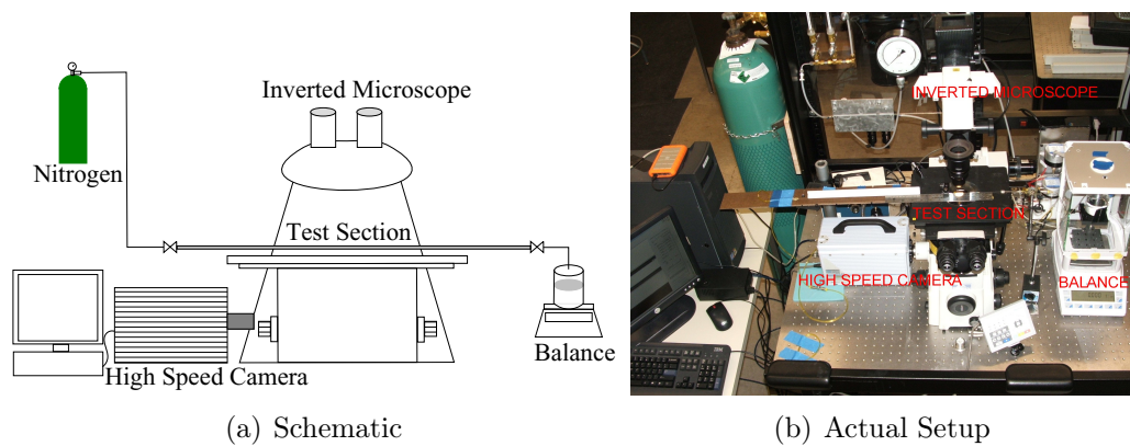
Figure 5.2. Film Measurements Setup
