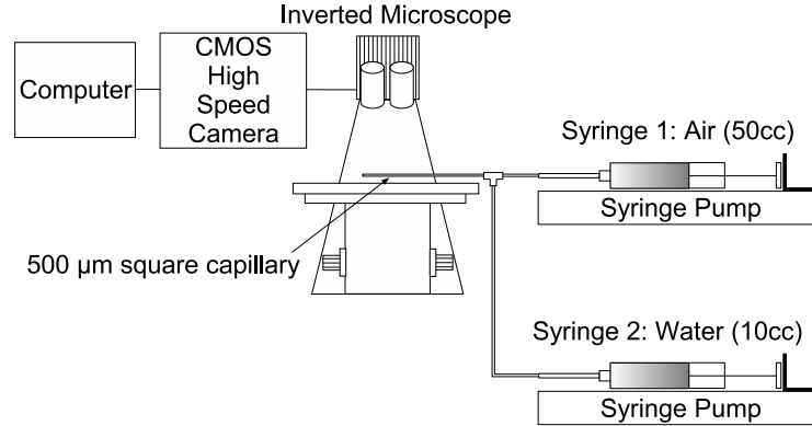
Figure 4.3. Schematic of high speed microscopy setup.
