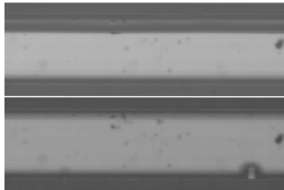
Figure 4.8. Top, separated flow in a square channel, \theta = 105^\circ . The bottom picture shows the channel with no flow. The flow is from right-to-left and the width of the images is 4.198 mm.
