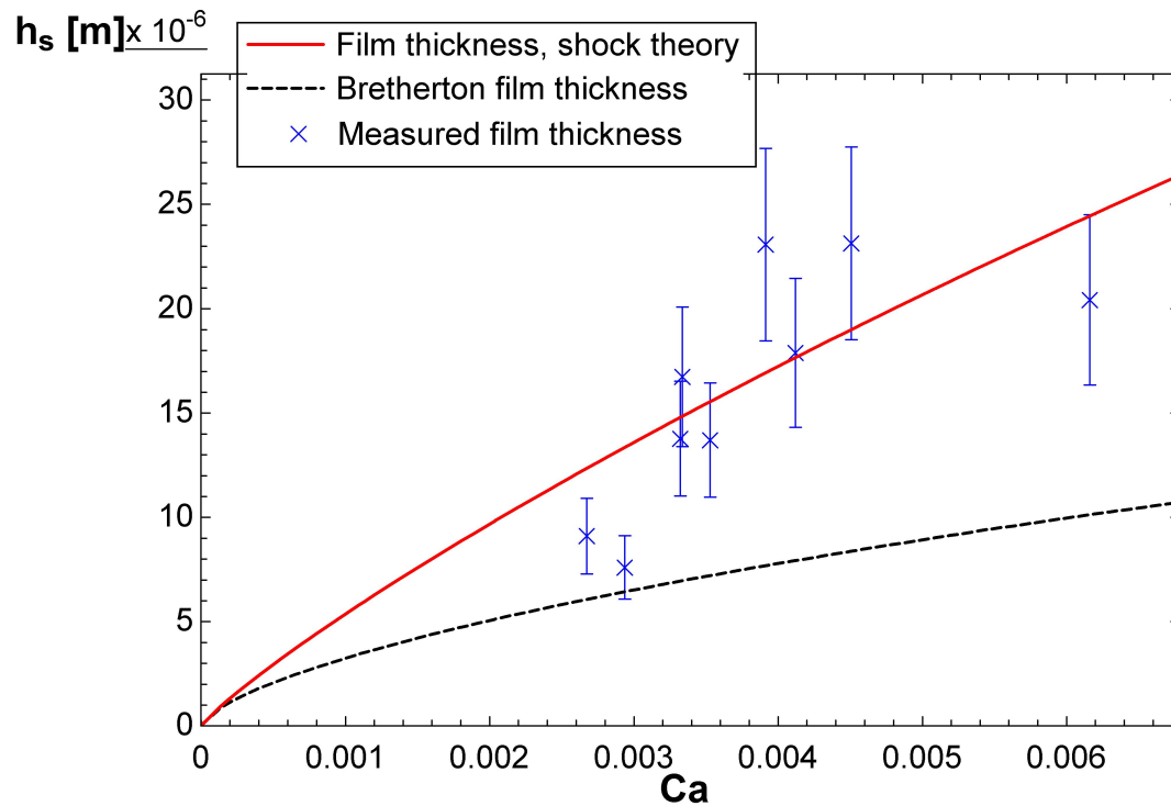
Figure 6.12. Non-wetting Film Thickness. The measured thickness follows the law obtained from the shock theory, except for the two leftmost data points which did not present a hydraulic jump. The wetting Bretherton film is shown for reference.
