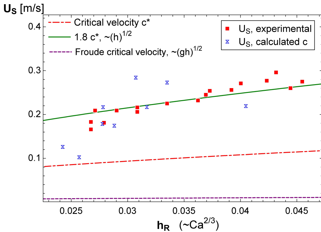
Figure 6.9. Shock Velocity vs. Nondimensional Film Thickness. U_S, experimental is the shock velocity measured in a number of separate runs in the non-wetting test section. U_S, calculated is the shock velocity computed with the shock theory relation Eqn. 6.3 using the measured film thickness. All data points lie above the critical shock velocity c^* which is computed using Eqn. 6.4. Bretherton's film thickness h_R dependency on Ca is given as a correlation by Aussillous and Quere [8].
