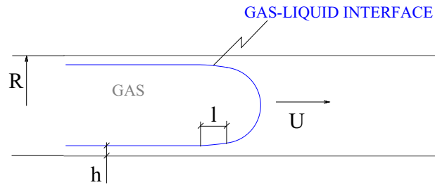
Figure 5.1. Film Deposition Schematic.
