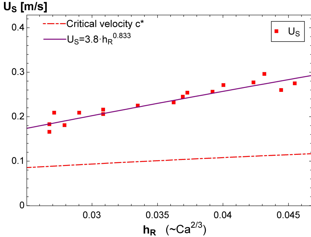
Figure 6.10. Shock Velocity vs. Non-dimensional Bretherton Film Thickness
