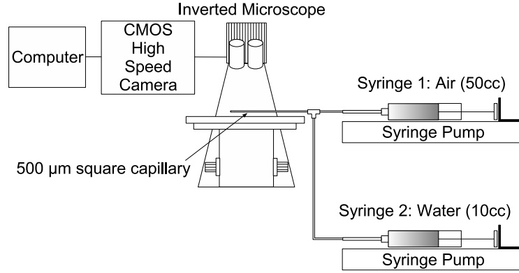
Figure 3.8. Schematic of high speed microscopy setup.
