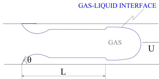
Figure 6.16. Non-Wetting Film Deposition with Hydraulic Jump
