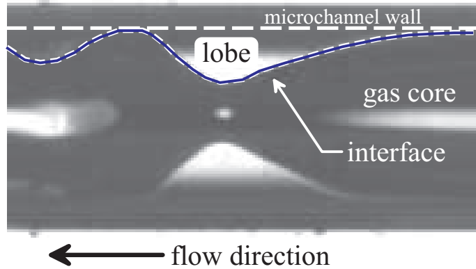
Figure 3.9. Image of lobe formation detailing the nozzle like liquid structure. The flow is from right-to-left with a high speed gas core. The bright areas of the image result from the unimpeded path of the backlight through the test section.
