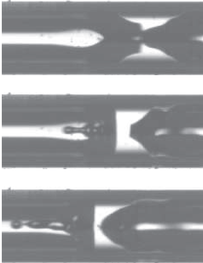
Figure 3.6. Magnified view of 2 ms droplet ejection sequence from Figure 3.5. In the top image (0.7 ms) coalescence is imminent. In the middle image (0.8 ms) coalescence has occurred and a liquid column is being ejected from the liquid plug. In the bottom image (0.9 ms) the liquid column is breaking up into drops which travel at very high velocities with the gas phase.
