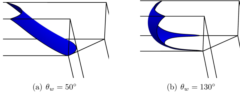
Figure 2.3. Critical volume plug in a 90^\circ bend of a square channel for \theta_b = 150^\circ on the GDL surface(lower horizontal plane). The interface curvature is positive for \theta_w = 50^\circ on the bipolar plate (vertical planes and upper surface) and the water is in a state of under-pressure with respect to the gas. For the nonwetting cases the curvature is negative with the water in a state of over-pressure with respect to the gas.
