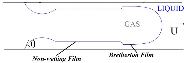
Figure 6.3. Hydraulic Jump Schematic. The thicker non-wetting film is separated by the Bretherton film through a hydraulic jump.
