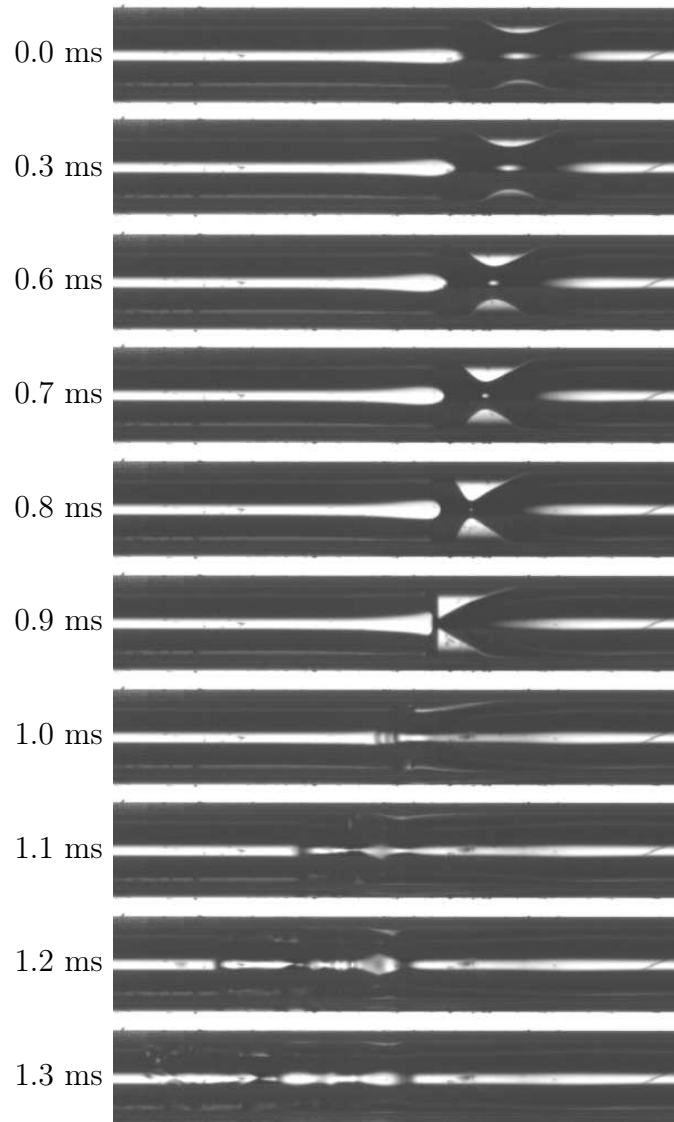
Figure 3.10. Sequence of lobe formation and collapse. The flow is from right-to-left and the width of the images is 3.931 mm.
